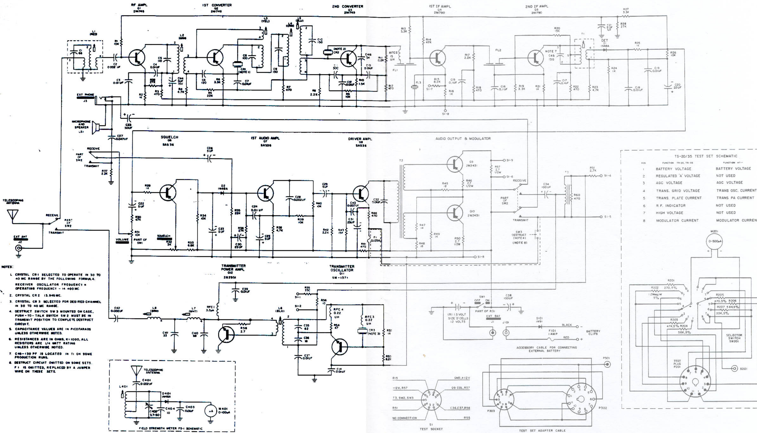
Figure 11. Model HT-1A Schematic Diagram.
