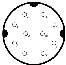
F90x/N90s connector front view
