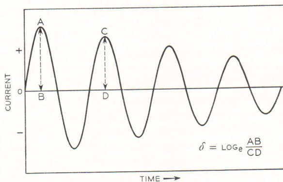
FIG. 2. Logarithmic decrement for damped wave-train.
