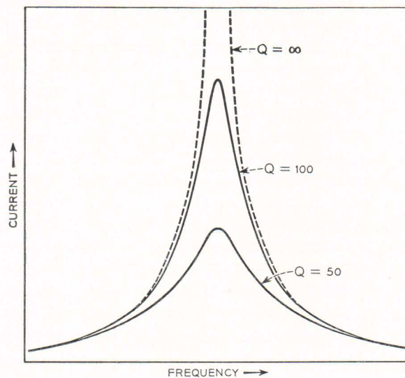
FIG. 1. Series resonance.
