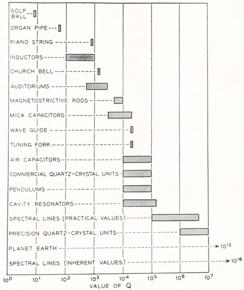
FIG. 3. Q's for various phenomena and devices.
