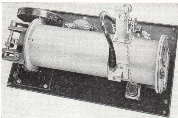
FIG. 5. Cavity resonator for radar testing
